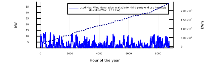
(Max. 13.3kW) Max. Wind Generation available for third-party end-use / markets (Installed Wind: 20.7 kW) (RHS: Cumulated (dot-line))
